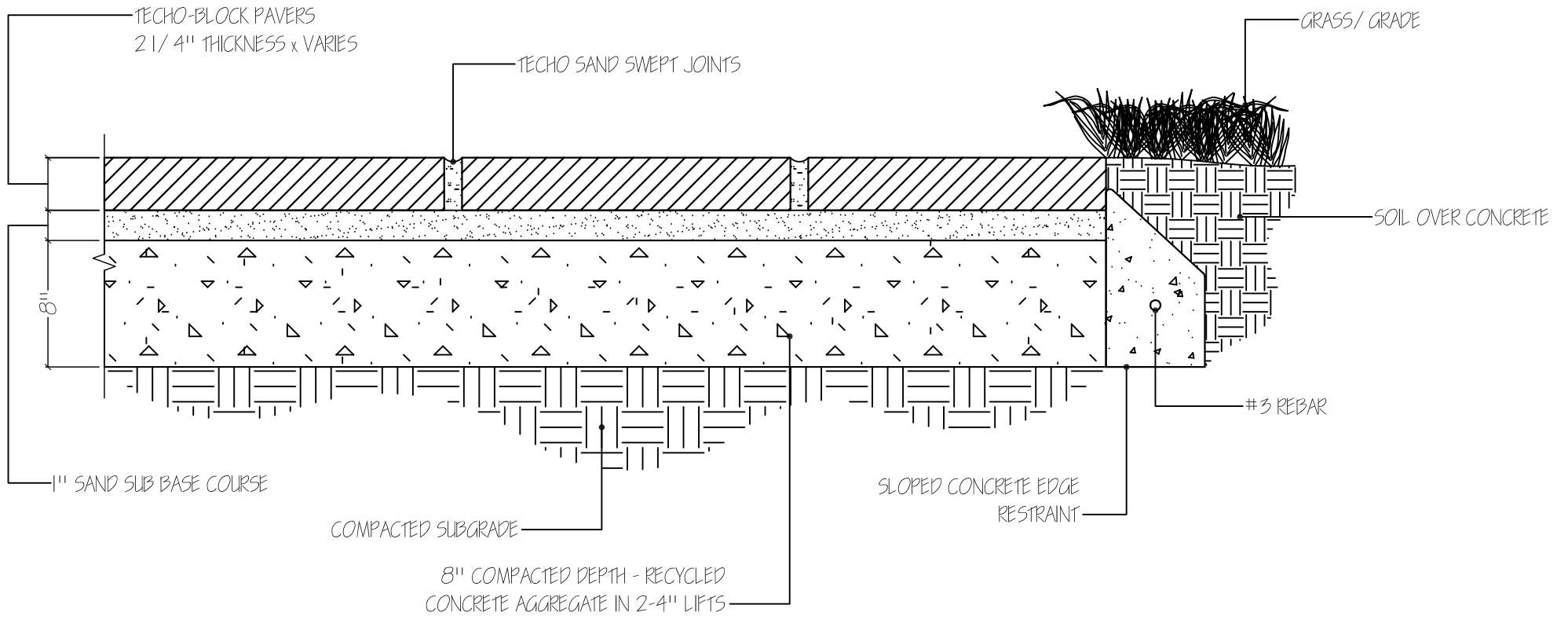
6 CONCRETE PAVER DETAIL Scale: NTS
